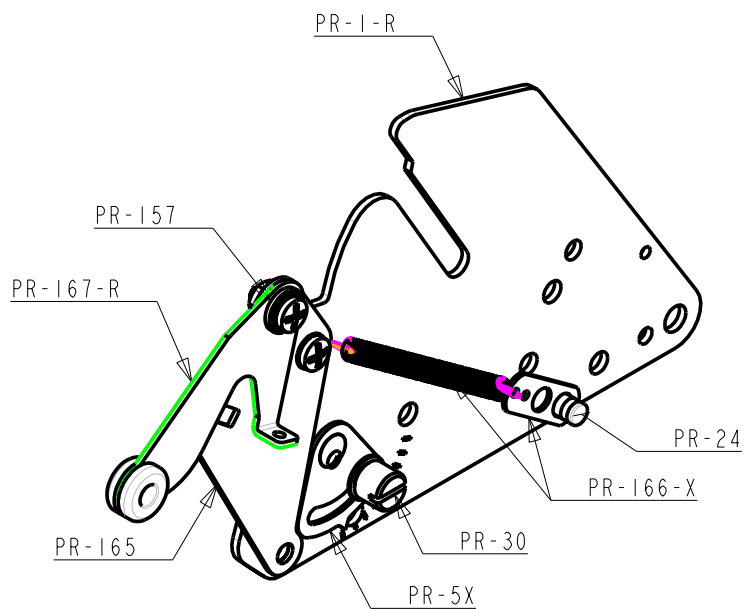
ITEM 2 PR-1RXX RIGHT FRAME ASSEMBLY
