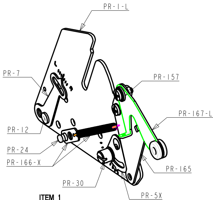
ITEM 1 PR-1LXX LEFT FRAME ASSEMBLY
