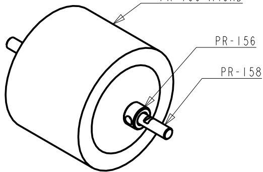
ITEM 3 - INK ROLL ASSEMBLY
